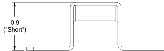
00CMK-0030-00 Cylinder Mounting Bracket, Short SCALE 1 : 1
