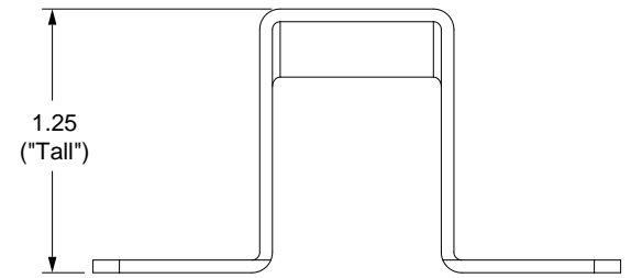
00CMK-0032-00 Cylinder Mounting Bracket, Tall SCALE 1 : 1
